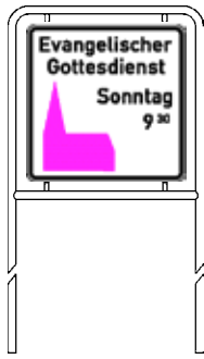
Standrohr-Ø 48,3/2,0 mm 750/750 mm
